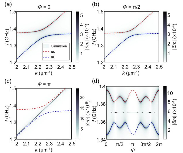
Figure 2 (Color online) The dispersion of magnon polarons formed by coupling between right-handed elastic waves and spin waves at different relative angles between magnon and phonon spin. The dashed colored curves represent theoretical dispersion relations obtained from eq. (17), while the background colormaps show numerical results of spin wave amplitude |\delta m| per unit volume. (a) Antiparallel alignment: \Phi = 0 , \mathbf{s}_p \cdot \mathbf{s}_m = -1 , showing maximum energy splitting. (b) Orthogonal alignment: \Phi = \pi/2 , \mathbf{s}_p \cdot \mathbf{s}_m = 0 , demonstrating reduced splitting. (c) Parallel alignment: \Phi = \pi , \mathbf{s}_p \cdot \mathbf{s}_m = 1 , exhibiting apparent null splitting due to dark mode excitation. (d) Angular dependence of energy splitting at resonant wave vectors as a function of relative angle \Phi , confirming the theoretical predictions.
