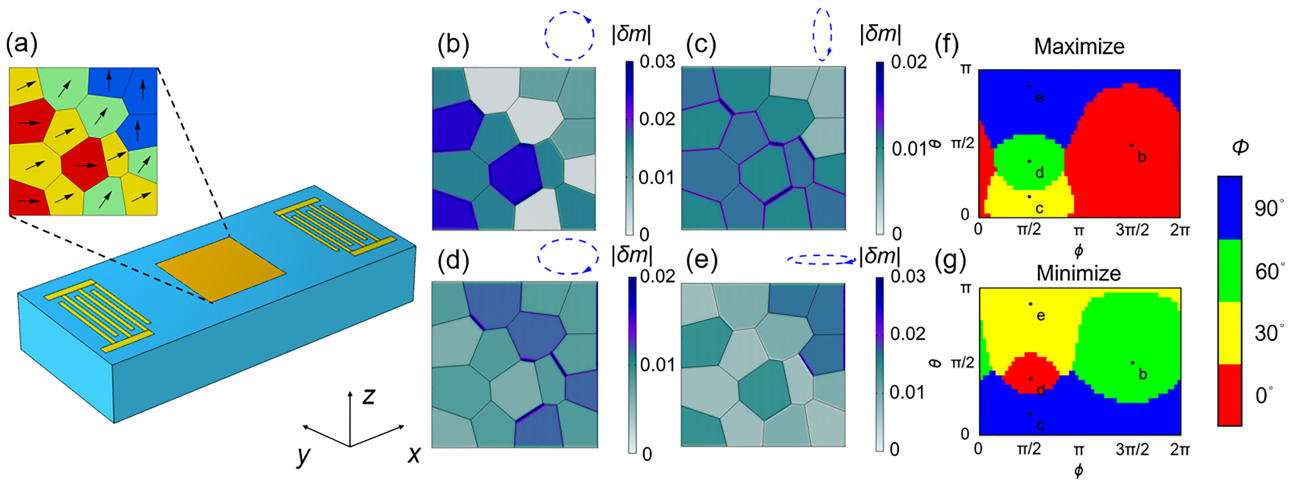
Figure 5 (Color online) (a) Schematic of BAW-driven magnon excitation in a multidomain YIG film (inset: domain map with easy-axis orientations). (b) Magnon excitation map under right-handed circular polarization ( \eta = 1 ). (c) Response under \eta = 5.8 . (d) Response under \eta = 0.68 . (e) Response under \eta = 0.42 . Insets in (b)–(e): polarization ellipses corresponding to each \eta . (f) and (g) Polarization sectors (red/green) that maximize or minimize total excitation intensity for domains oriented at 0^\circ and 60^\circ , respectively.
