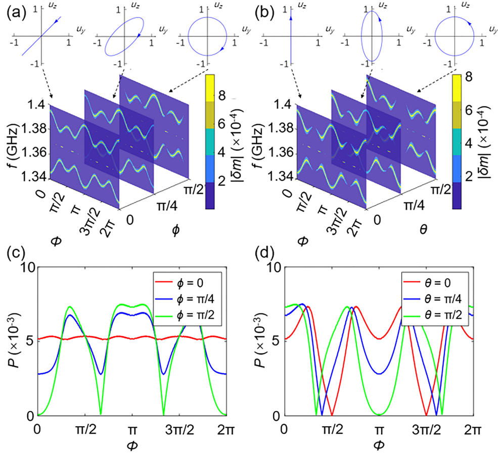
Figure 3 (Color online) Magnon excitation efficiency under elastic wave driving with variable phonon spin configurations. (a) Magnon excitation spectra driven by elastic waves with fixed amplitude parameter \theta = \pi/2 and variable phase parameter \phi \in \{0, \pi/4, \pi/2\} , demonstrating phase-dependent magnon resonance activation (top insets show corresponding elastic wave polarization ellipses). (b) Complementary analysis of magnon excitation under elastic wave driving with fixed phase \phi = 3\pi/2 and variable amplitude ratio \theta \in \{0, \pi/4, \pi/2\} (polarization geometries shown above). (c) and (d) Total excitation intensity P as a function of spin misalignment angle for configurations in panels (a) and (b), respectively.
